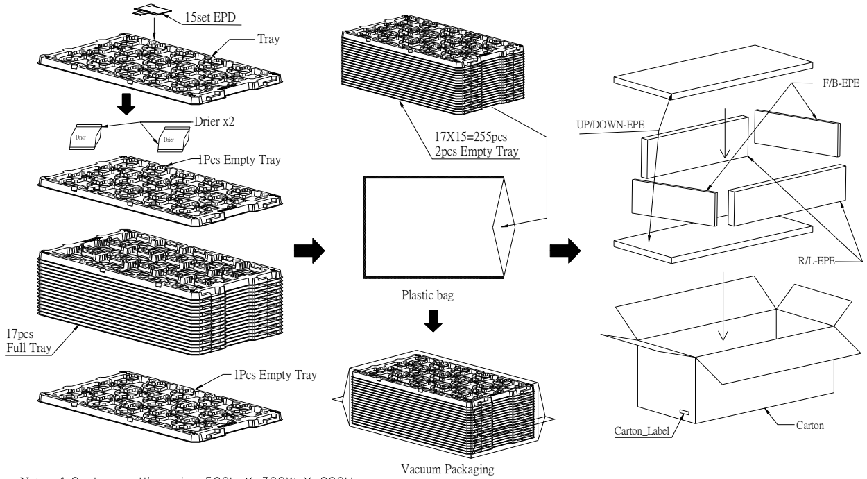
Figure 7-1 Packing Diagram
