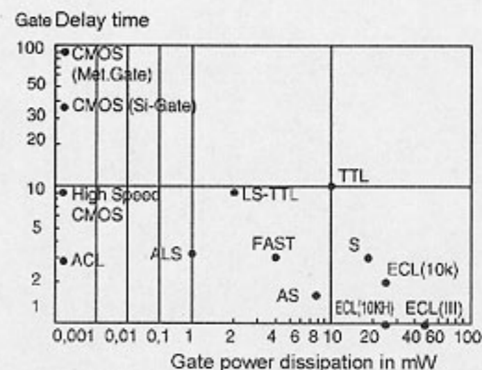
Speed x Power dissipation TTL/CMOS-Families
