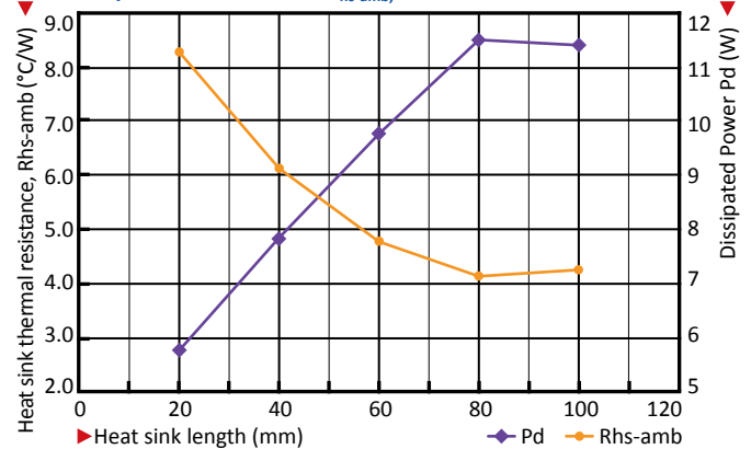
XSA-215 performance data at a heat sink to ambient temperature difference, ΔT hs-amb , of 50 °C
