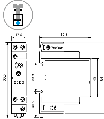
80.71 Screw terminal
