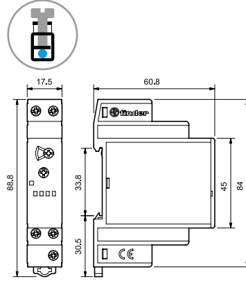
80.41 Screw terminal
