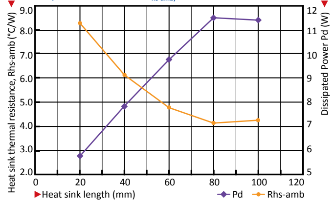
XSA-216 performance data at a heat sink to ambient temperature difference, \Delta T_{hs-amb} , of 50^{\circ}\text{C}
