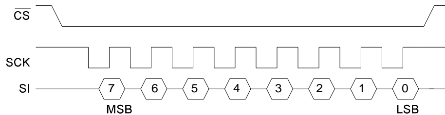
Figure 4. SPI Modes 0 & 3
