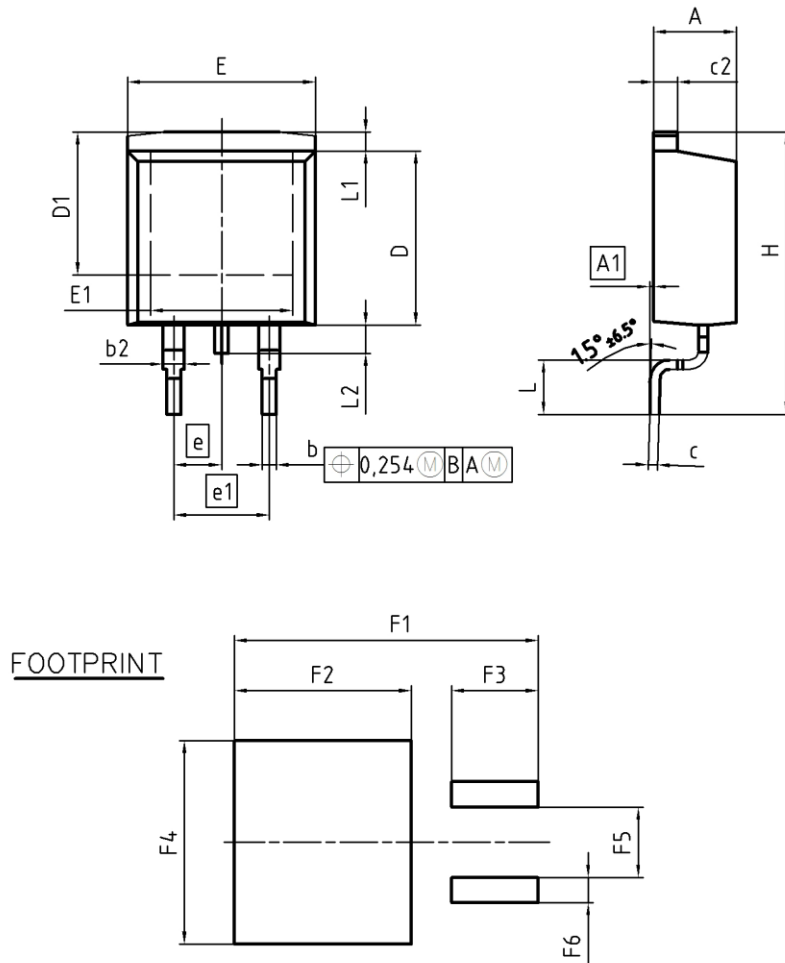
PG-TO263-3
