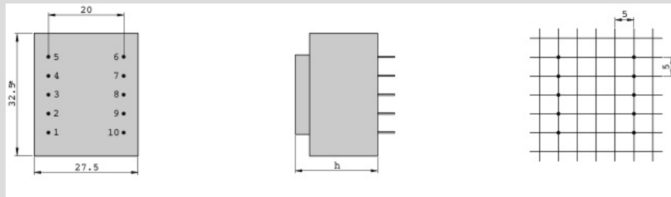
Dimensions without tolerance \pm 0.3 mm Design changes reserved
