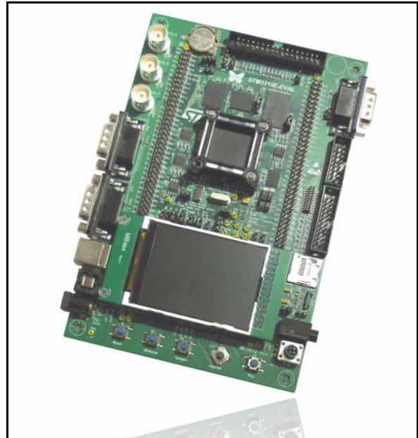
Figure 1. STM3210E-EVAL evaluation board
