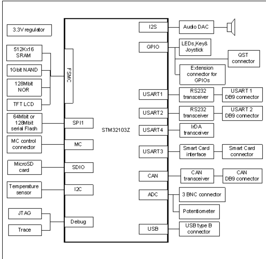
Figure 2. Hardware block diagram
