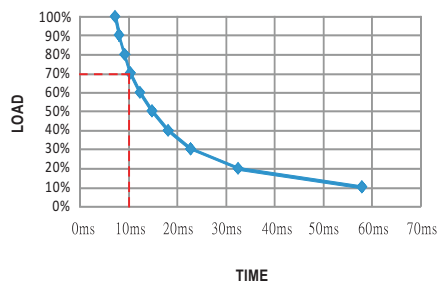
RSD-150C-12
