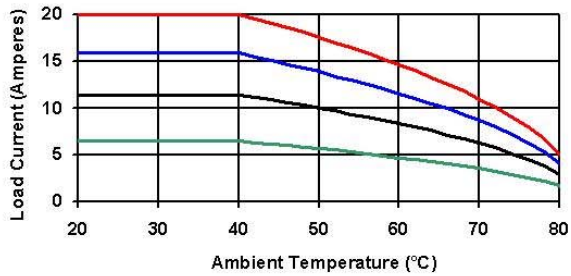
Derating Curve: DC400D10
