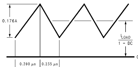
10 µH Inductor Current, 5V–12V Boost (LM2731X)
