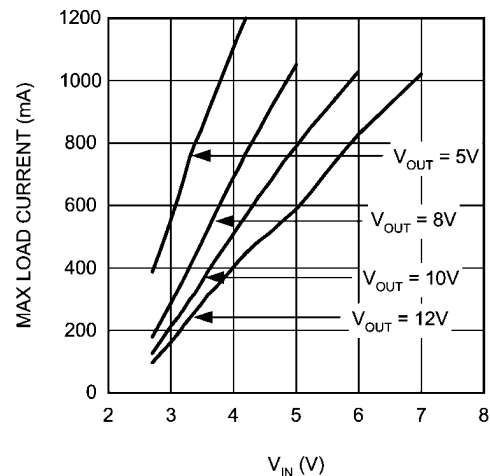
Max. Load Current (typ) vs V_IN - "Y"
