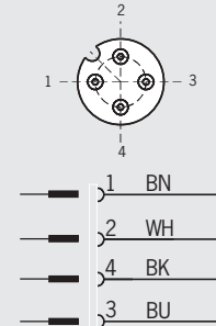
Wiring diagram (view of connection side)
