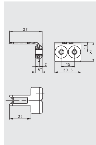
Actuator M-WT bent Rubber bush, overtravel 4 mm
