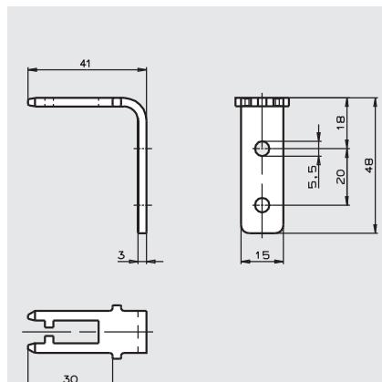
Actuator P-W bent overtravel 2 mm
