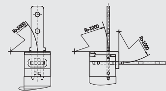
Minimum door radii with insertion funnel
