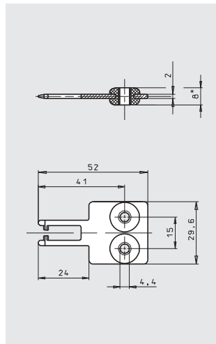
Actuator M-GQ straight Transverse rubber bush, overtravel 4 mm
