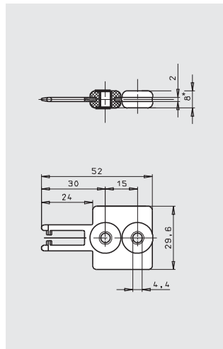
Actuator M-GT straight Longitudinal rubber bush, overtravel 4 mm
