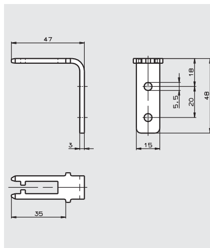
Actuator P-WN bent overtravel 7 mm
